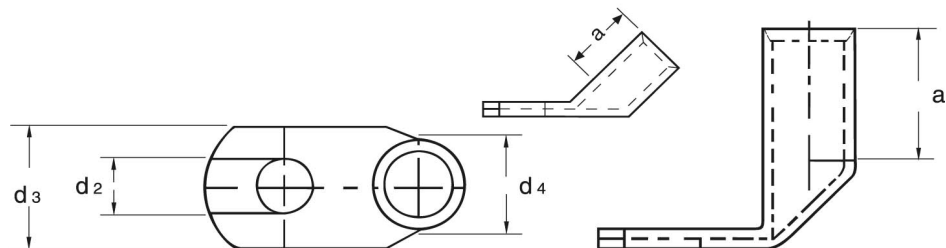
angle cable-lugs
